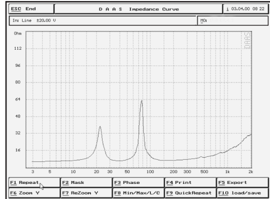
Impedance curve
