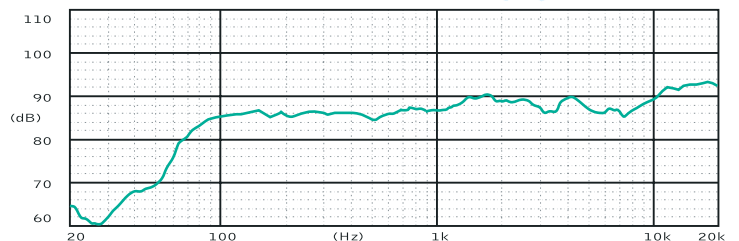
Frequency Response
