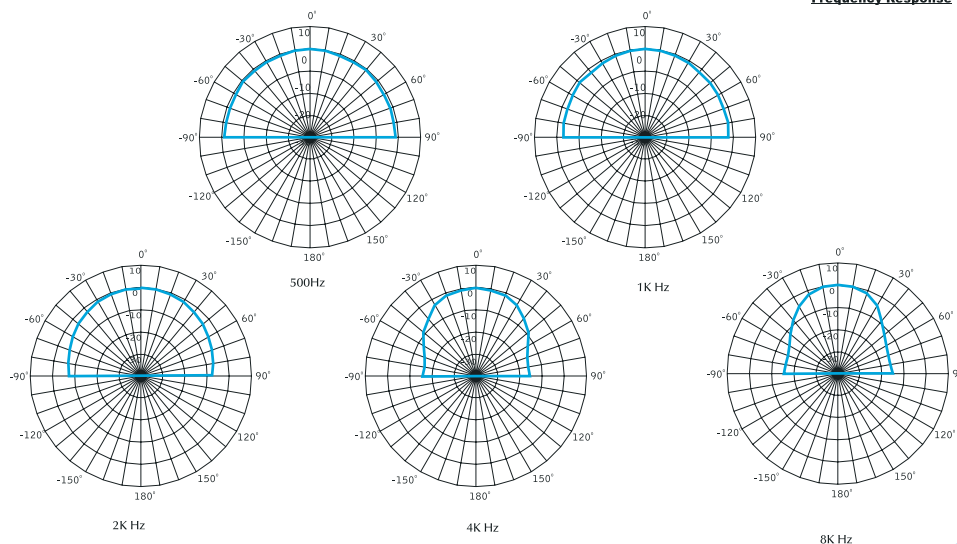
Polar Pattern
